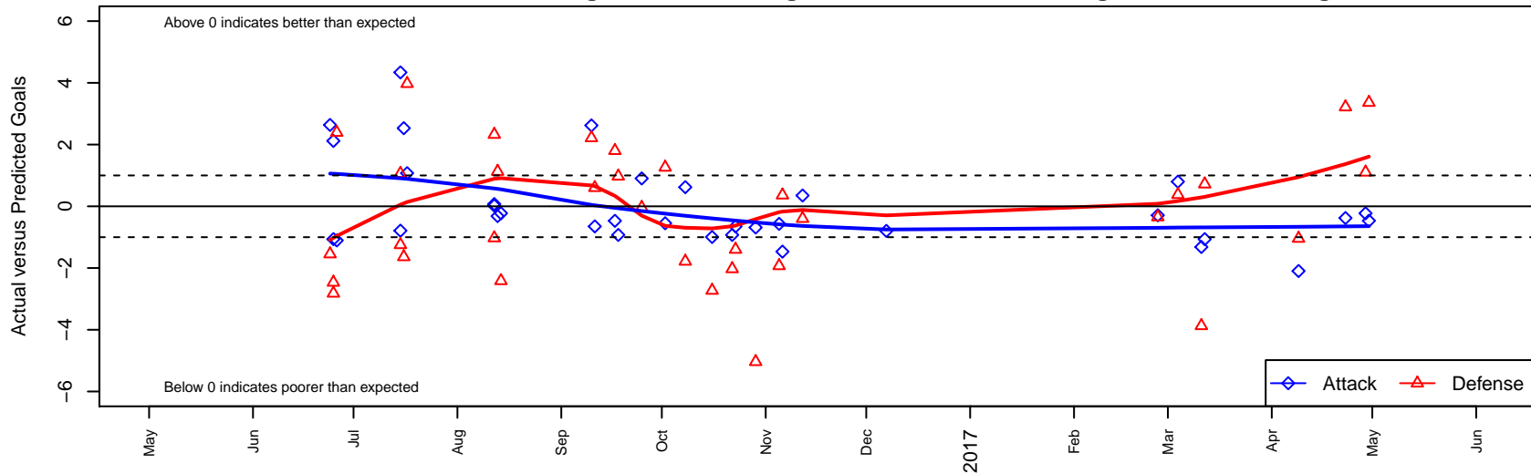
CSC Storm White B05 Dots are actual minus expected GF (blue circles) and GA (red triangles). Blue line is smoothed change in attack strength. Red is smoothed change in defense strength.
